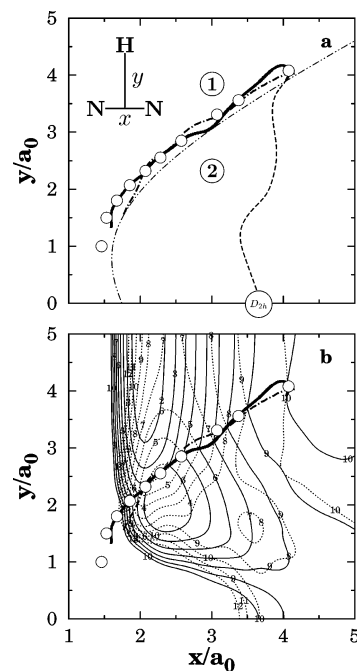
Figure 7. T-shaped crossing seam. Key for panel a: (○) calculated points; (---) as obtained from fitted diagonal states; (—) as obtained from fitted adiabatic states without the damping function in eq 53; (—) as obtained from fitted adiabatic states with the above damping function. The dashed-dot (— · —) represents the x_0(x) curve in eq 50. The numbers label the regions referred to in the text, while the large open circle indicates the D_{2h} conical intersection of the adiabatic states. Panel b shows also energy contours for the ground (—) and excited (---) states, in both cases starting at E_0 = -0.3641E_h and equally spaced by \Delta E_0 = 0.0385E_h .
