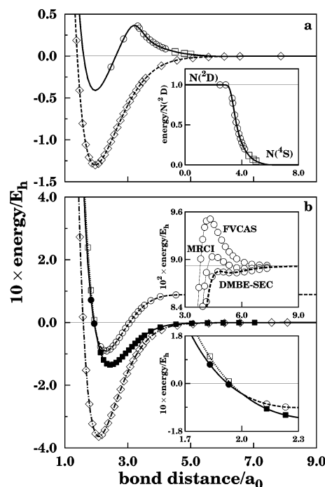
Figure 5. EHFACE2U potentials energy curves. Key for panel a : ( \circ ) \text{HN}_2(2^2A') with r_{\text{NN}} fixed at 8a_0 forming an angle \theta_{\text{HNN}} with the r_{\text{NH}} axis fixed at = 5^\circ ; ( \diamond ) \text{NH}(^3\Sigma^-) ; ( \square ) \text{NH}(^3\Sigma^-) ; (—) \text{NH}(^3\Sigma^-)(R) + h(R) ; (---) \text{NH}(^3\Sigma^-)(R) . The solid lines in the insets show h(R) , with all points referred to the \text{NH}(^3\Sigma^-) diatomic. Key for panel b : ( \circ ) \text{N}_2(^3\Pi_g) ; ( \diamond ) \text{N}_2(^3\Sigma_u^+) ; ( \square ) \text{N}_2(^3\Sigma_u^+) ; (---) \text{N}_2(^1\Sigma_g^+)(R) ; (---) \text{N}_2(^3\Pi_g)(R) ; (---) \text{N}_2(^3\Sigma_u^+)(R) . Filled symbols have been used to calibrate k(x) , with the solid lines showing \text{N}_2(^3\Pi_g)(R)k(R) + \text{N}_2(^3\Sigma_u^+)(R)[1 - k(R)] .
